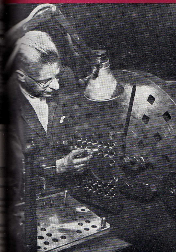
Turner J. Campbell turning an Oil Seal Bush, 49-cavity mould.
