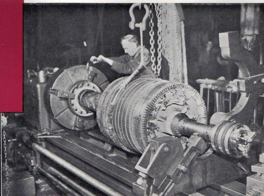
Here is Turner W. Laing at work on the Slip Rings of our Bunbury Motor, which were recently turned up.
